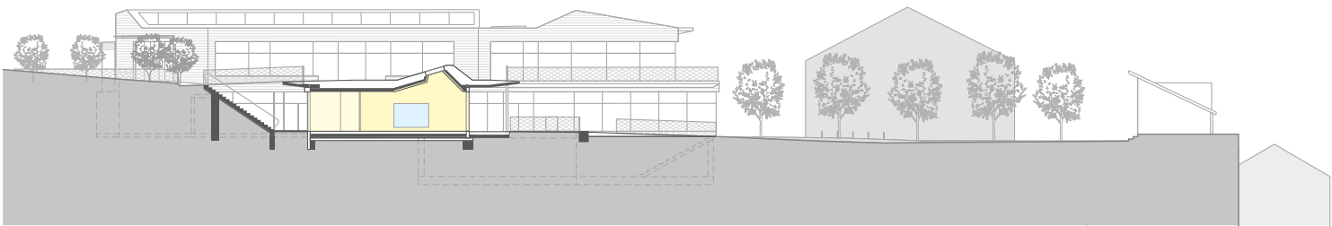
SNITT KINDERGARTEN
